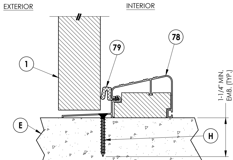
3 VERTICAL CROSS SECTION 5 Outswing shown
