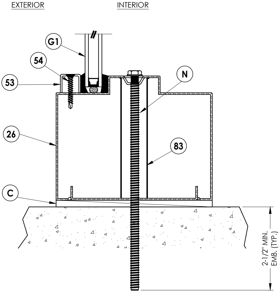
2 6 VERTICAL CROSS SECTION
